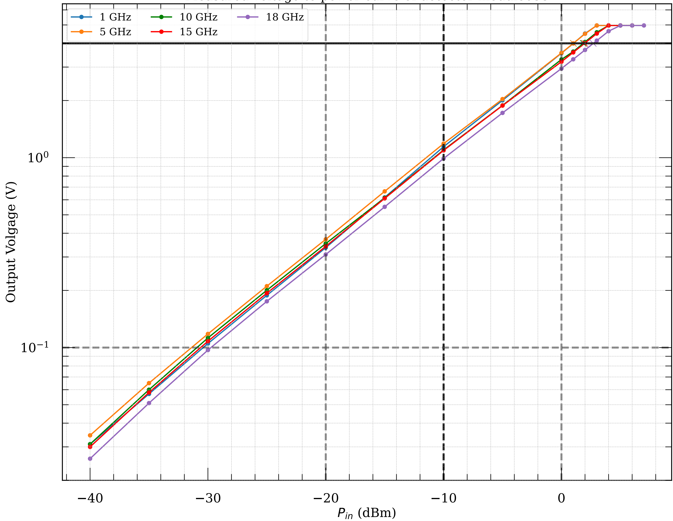
Measured voltage-to-power curve of detector module058
